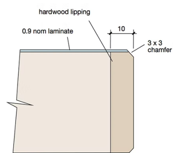
Laminate Face, Concealed Lipping
