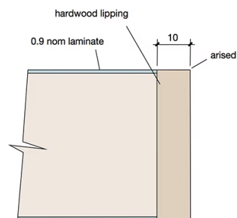
Laminate Face, Exposed Lipping
